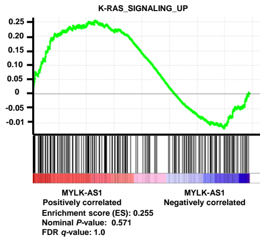
Supplementary Figure 1. GSEA analysis of MYLK-AS1 in HCC adjacent normal tissues. Cluster analysis of MYLK-AS1 did not correlate with the activation of K-RAS signaling in HCC adjacent normal tissues.
