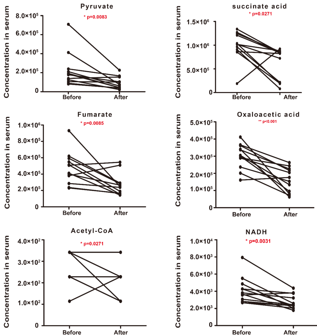
Supplementary Figure 1S. The metabolism profile indicated the decreasing of metabolites in NSCLC brain metastasis patients' blood serum after CyberKnife Stereotactic Radiotherapy. Significance was assessed with paired t-tests. *P<0.05. **P<0.01, *** P<0.001.
